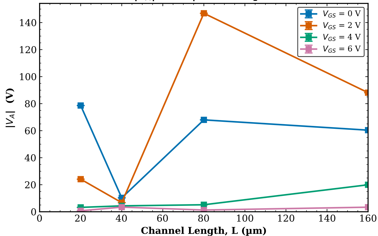
TFT2 Transistor 1 |V_A| vs L | W = 10\text{ }\mu\text{m}
